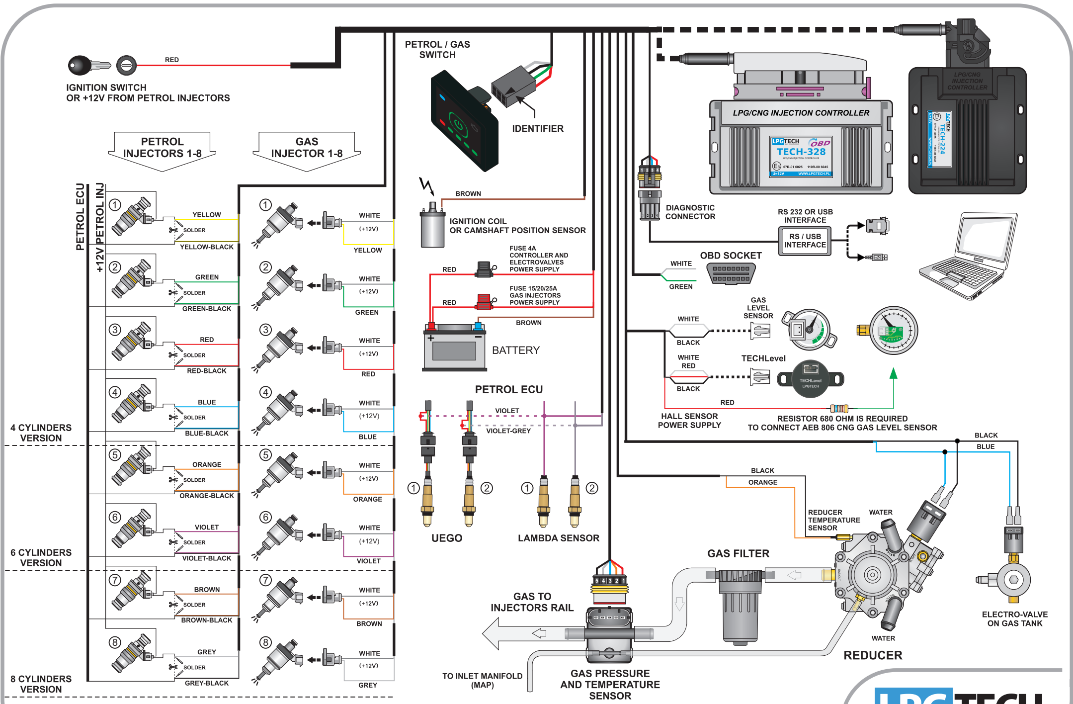
TECH Controllers - connection diagram
